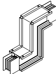
FLATWISE OFFSET
