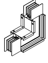
FLATWISE ELBOW
