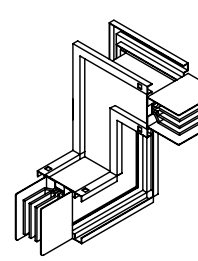
COMBINATION ELBOW
