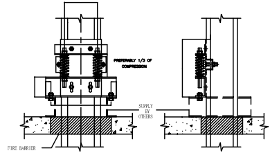
VERTICAL SPRING HANGER
